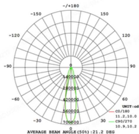
INTENSITY DISTRIBUTION DIAGRAM IN C PLANS
