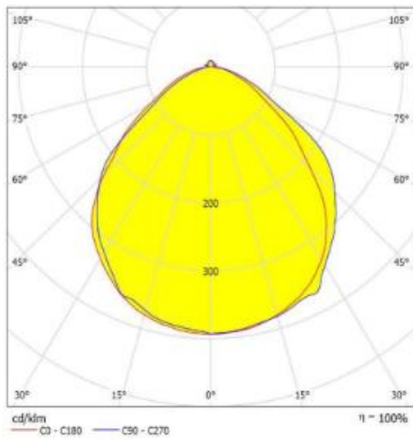
Luminance Distribution
