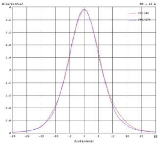
Illumination Curve
