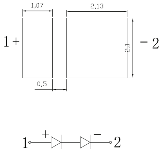
Figure 9b. Recommended PCB solder pad layout for L128-xxxxRB35000A1, L128-xxxxRC35000A1, L128-xxxxRC35000B1, L128-xxxxRC35000C1, L128-xxxxRD35000A1, L128-xxxxRD35000B1, and L128-xxxxRE35000A1..
