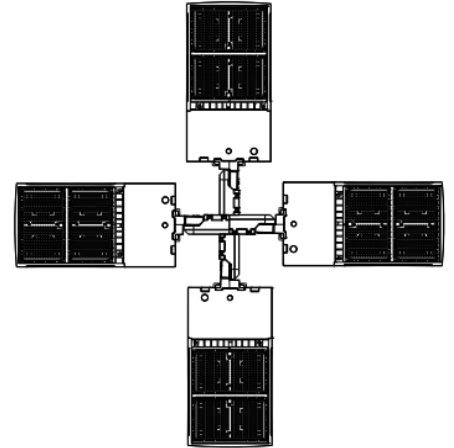
Q90 Quad90° EPA: 2.18 Weight :79.2 lbs
