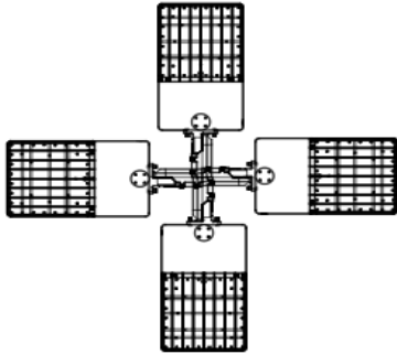
Q90 Quad 90° EPA:1.2 Weight:65.2 lbs.
